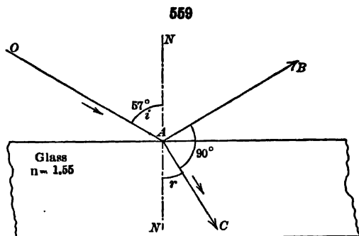
Brewster's Law
